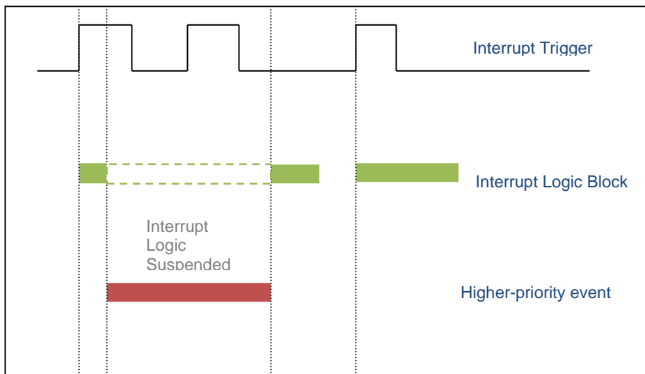
Figure 70: Interrupt Execution Considerations
