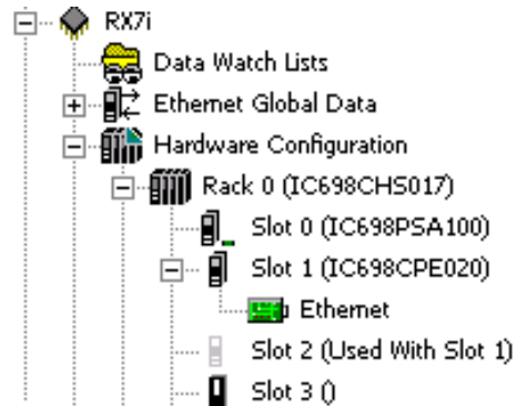
Figure 41: PME Expansion of PACSystems Target
