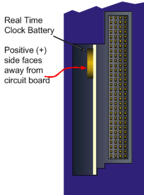
Figure 30: Accessing Real-Time Clock Battery (CPE302, CPE305 and CPE310)
