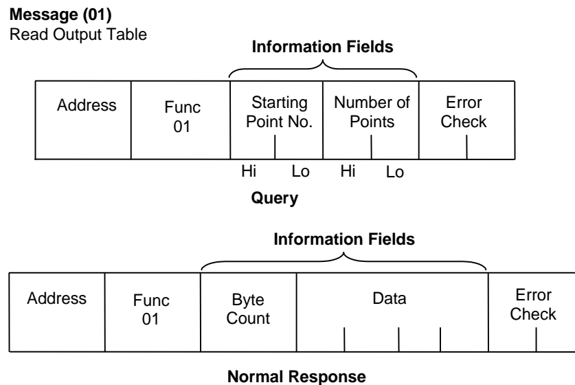
Figure 55: RTU Read Output Table Example
