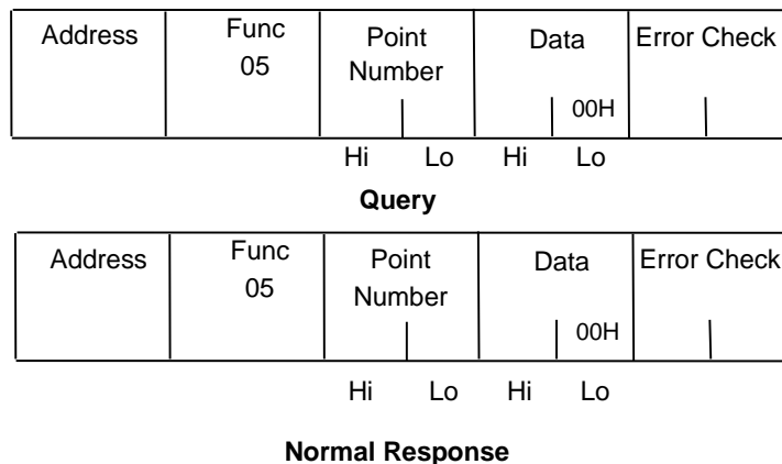
Figure 61: RTU Force Single Output Message Format
