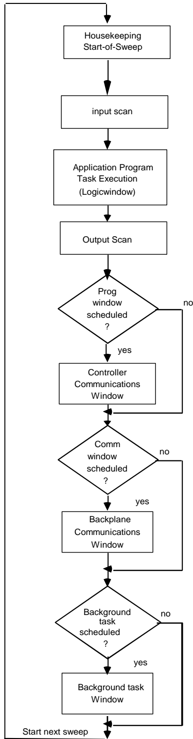
Figure 45: Major Phases of a Typical CPU Sweep
