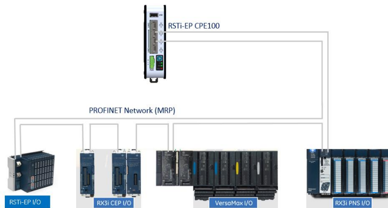
Figure 40: Typical Multi-Tier LAN Application (Ring Topology)
