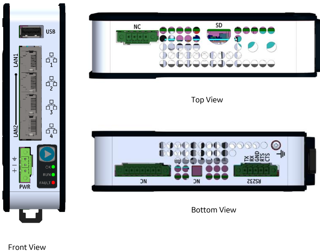
Figure 36: CPE100 Front, Top and Bottom Views and Features
