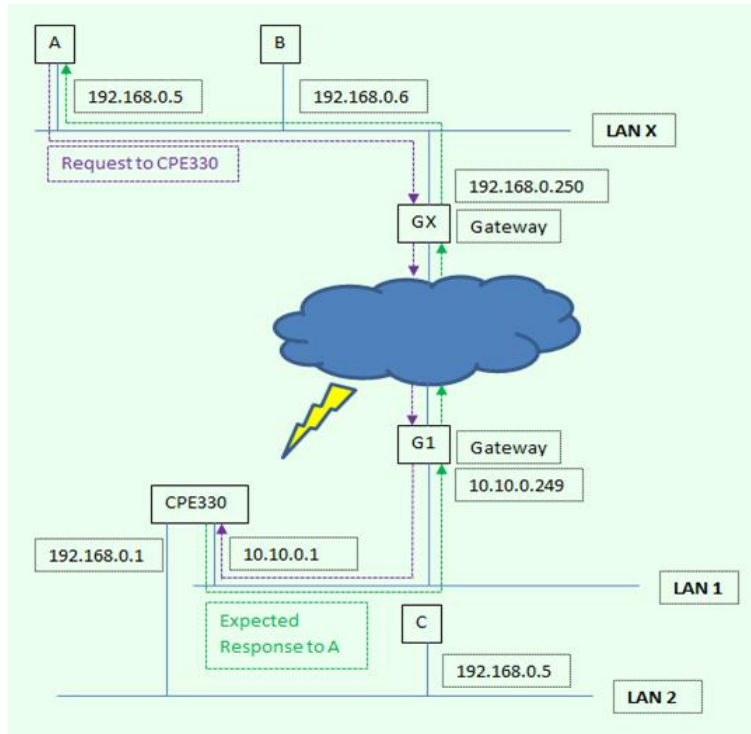
Figure 51: Expected Response Path
