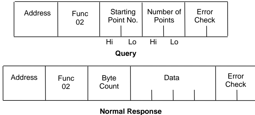
Figure 58: RTU Read Input Table Message Format
