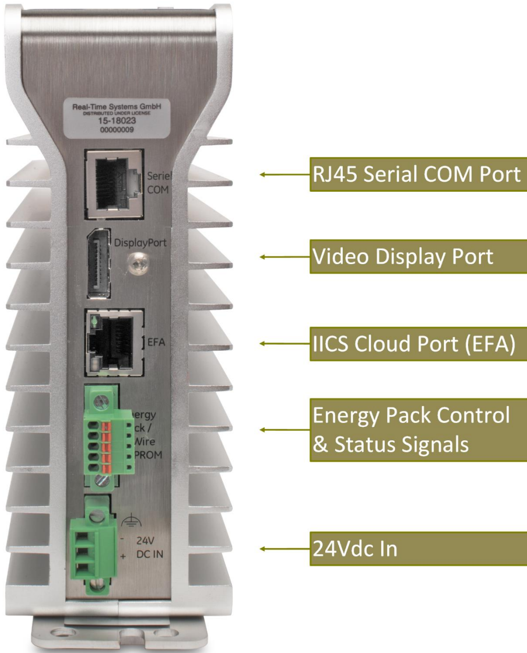
Figure 8: CPE400 Underside Ports & Connectors
