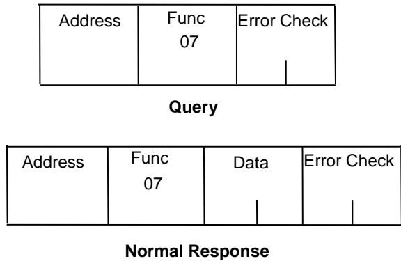
Figure 63: RTU Read Exception Status Message Format
