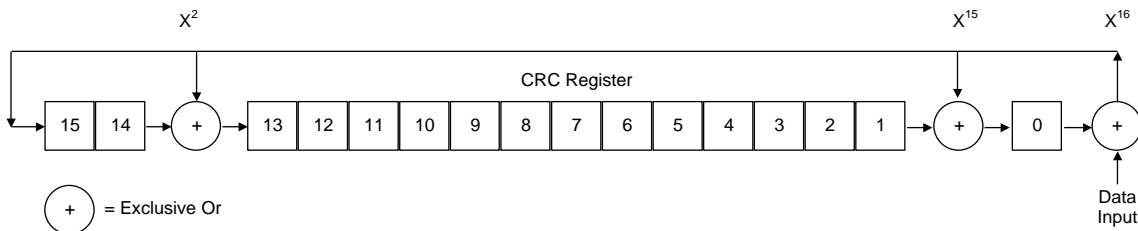
Figure 56: CRC Register Operation
