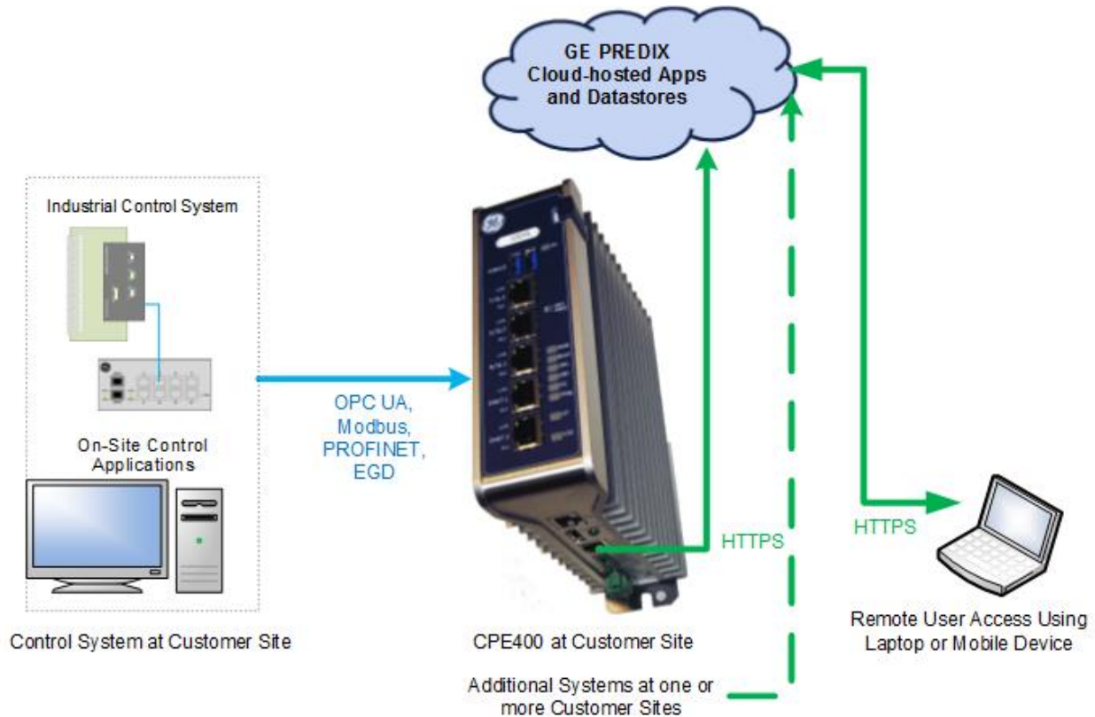
Figure 10: Typical Field Agent Application
