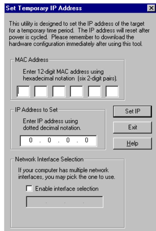
Figure 44: Set Temporary IP Address
