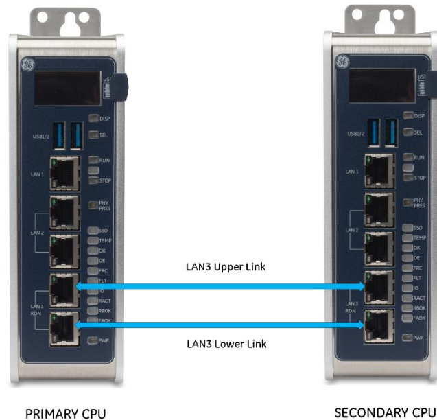
Figure 18: LAN3 Interconnects for Hot Standby Redundancy
