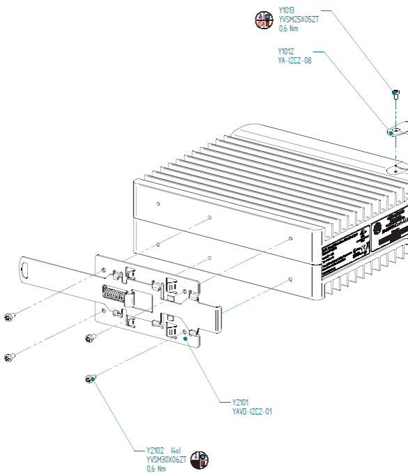
Figure 21: DIN-Rail Mount Bracket Assembly CPE400
