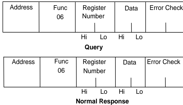
Figure 62: RTU Preset Single Register Message Format
