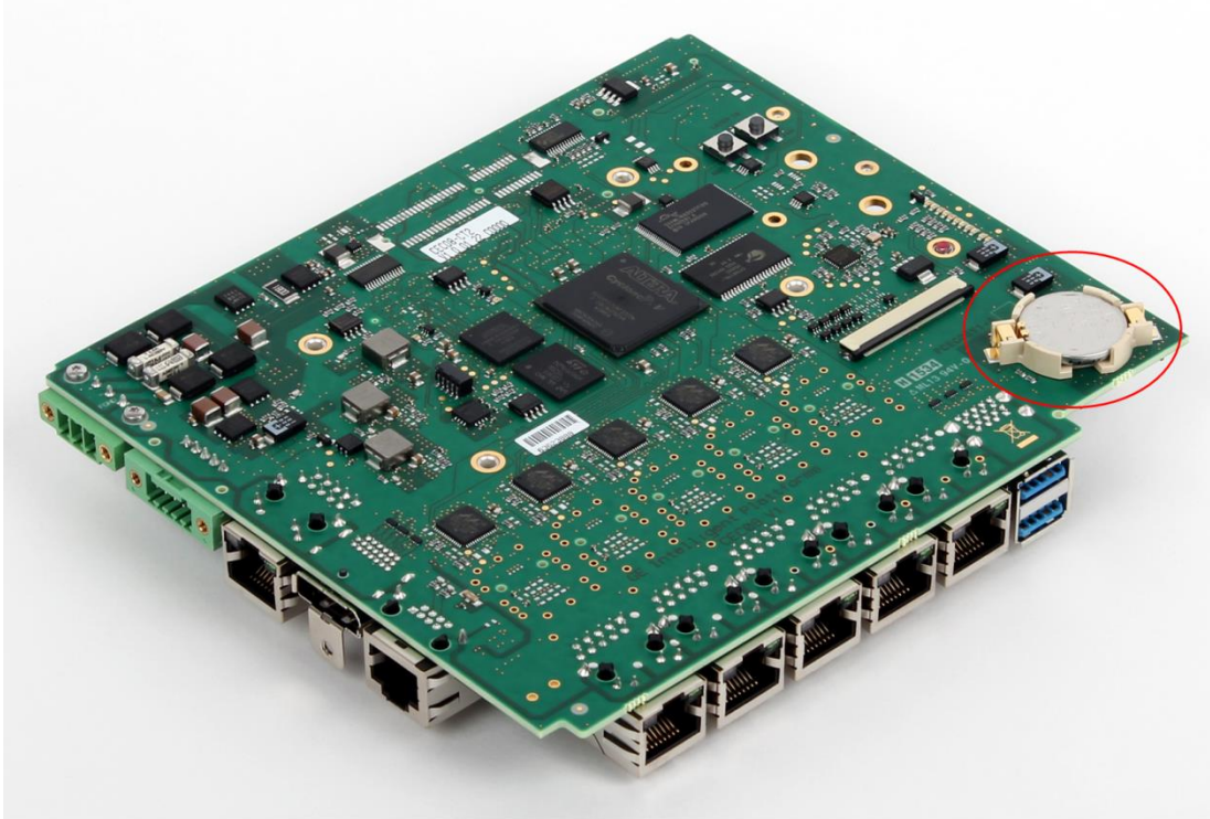
Figure 20: Location of RTC battery on CPE400
