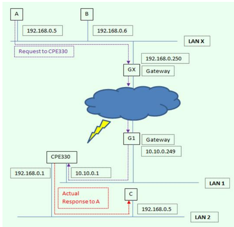
Figure 52: Actual Response Path
