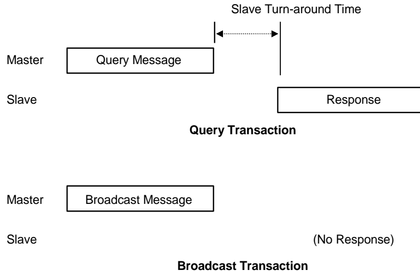
Figure 54: RTU Message Transactions
