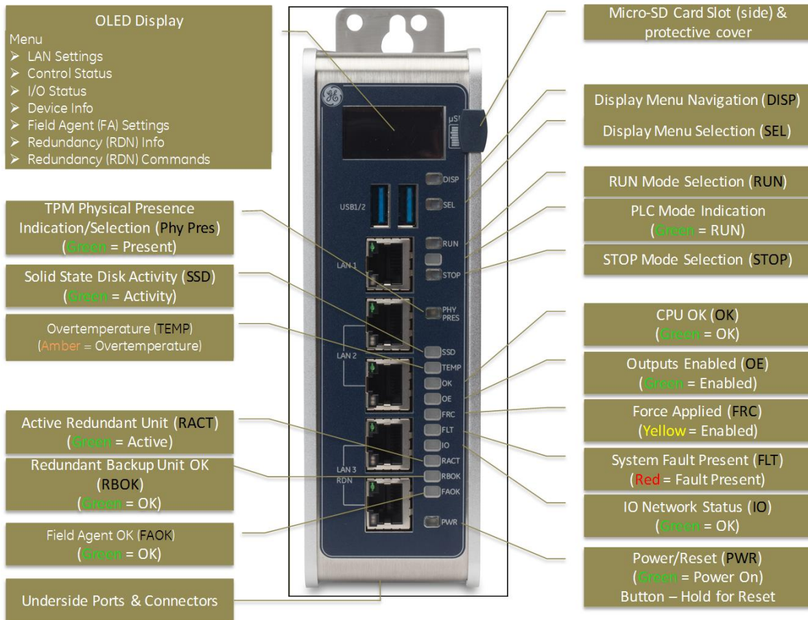
Figure 7: CPE400 Front View and Features
