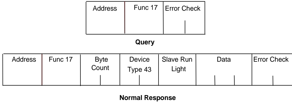
Figure 67: RTU Report Device Type Message Format
