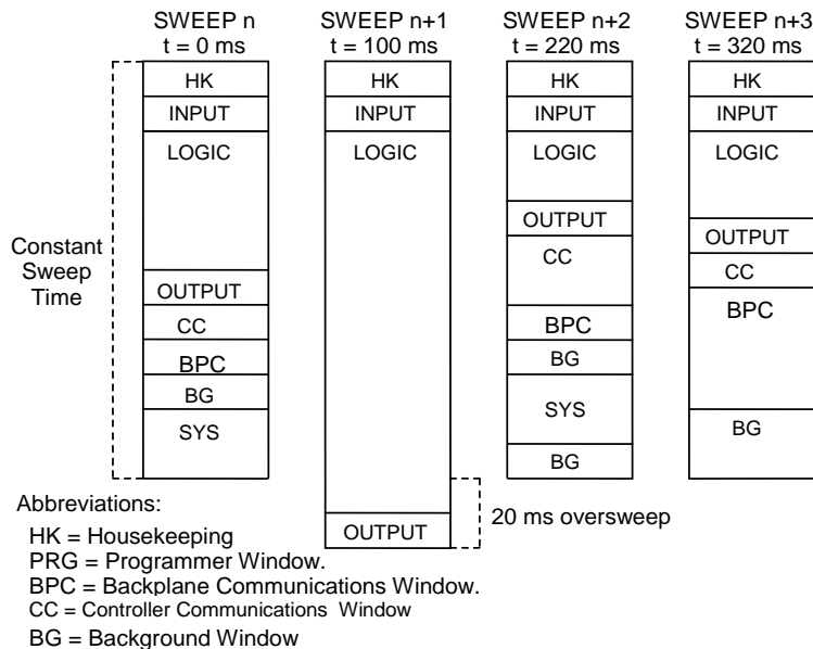
Figure 47: Typical Sweeps in Constant Sweep Mode
