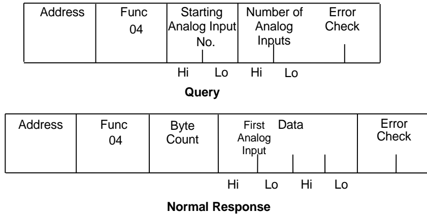
Figure 60: RTU Read Analog Inputs Message Format
