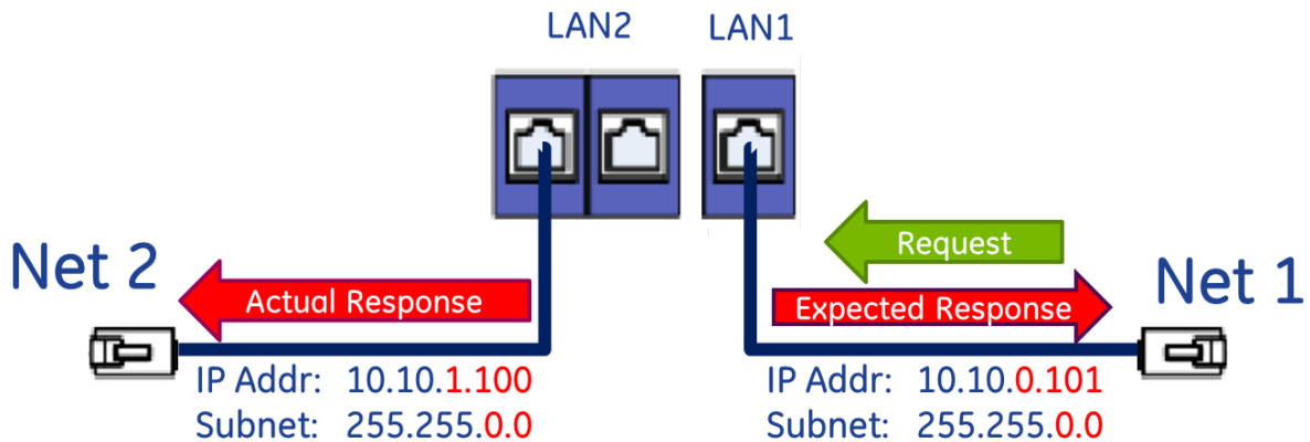
Figure 50: CPE330 Overlapping Local IP Subnet Example
