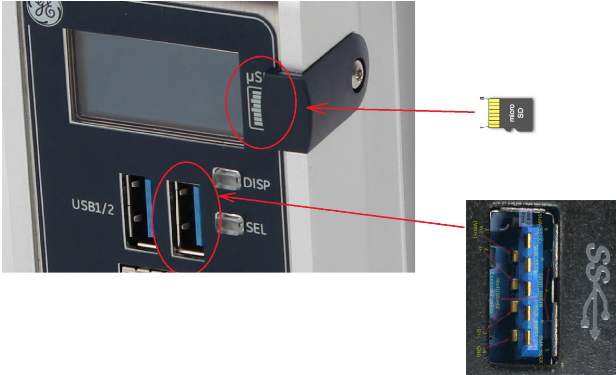
Figure 9: CPE400 Micro-SD & USB Pinouts
