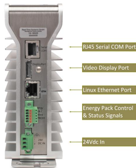
Figure 4: Underside Ports & Connectors 46
