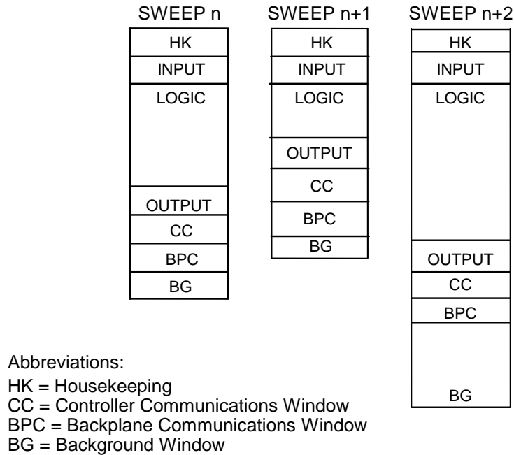
Figure 46: Typical Sweeps in Normal Sweep Mode
