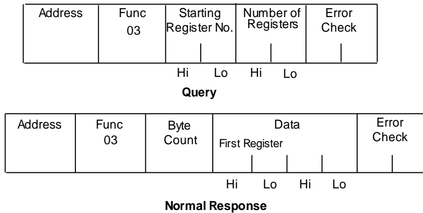
Figure 59: RTU Read Registers Message Format
