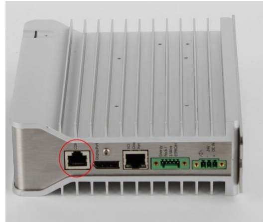
Figure 53: COM1 Port CPE400/CPL410
