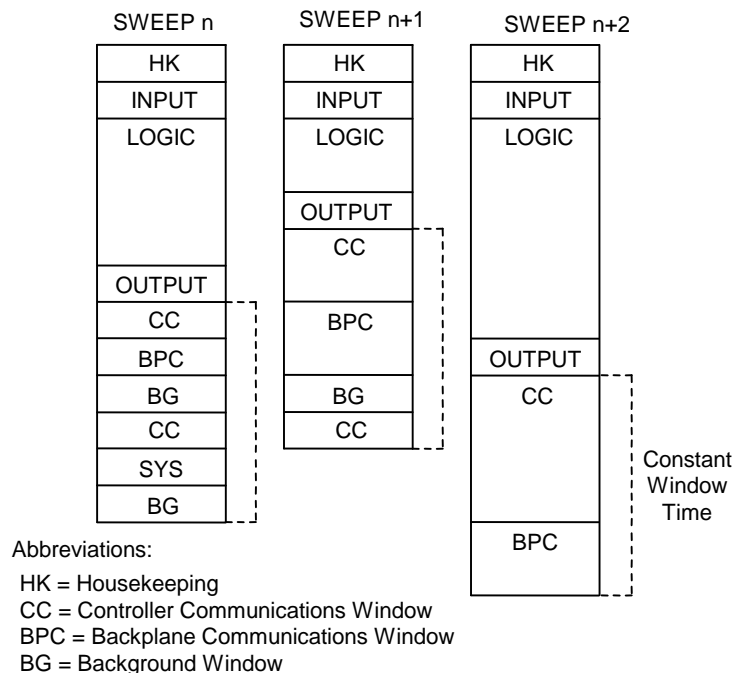
Figure 48: Typical Sweeps in Constant Window Mode
