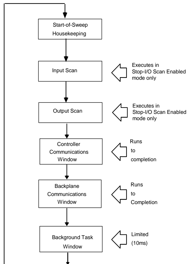
Figure 49: CPU Sweep in Stop-I/O Disabled and Stop-I/O Enabled Modes
