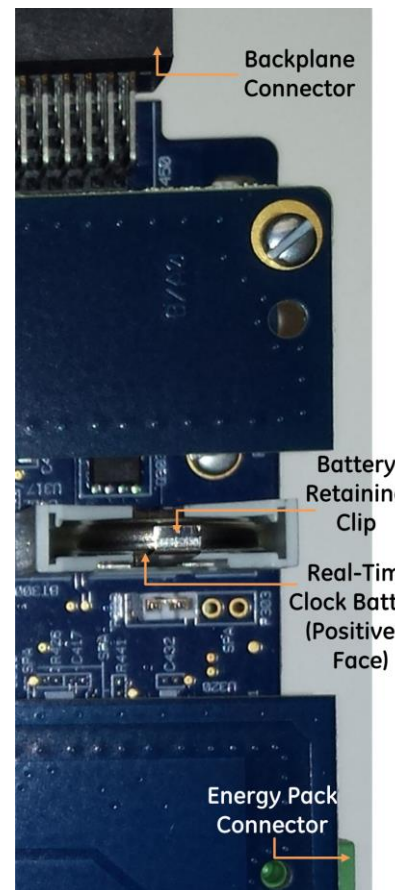
Figure 25: Location and Orientation of Real-Time Clock Battery in CPE330
