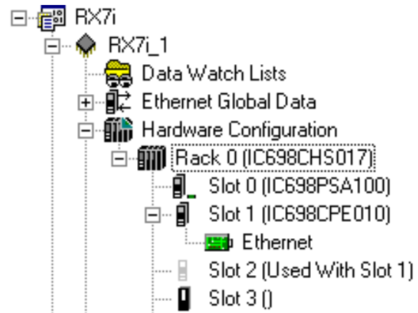
Figure 43: Selecting Embedded Ethernet for Configuration
