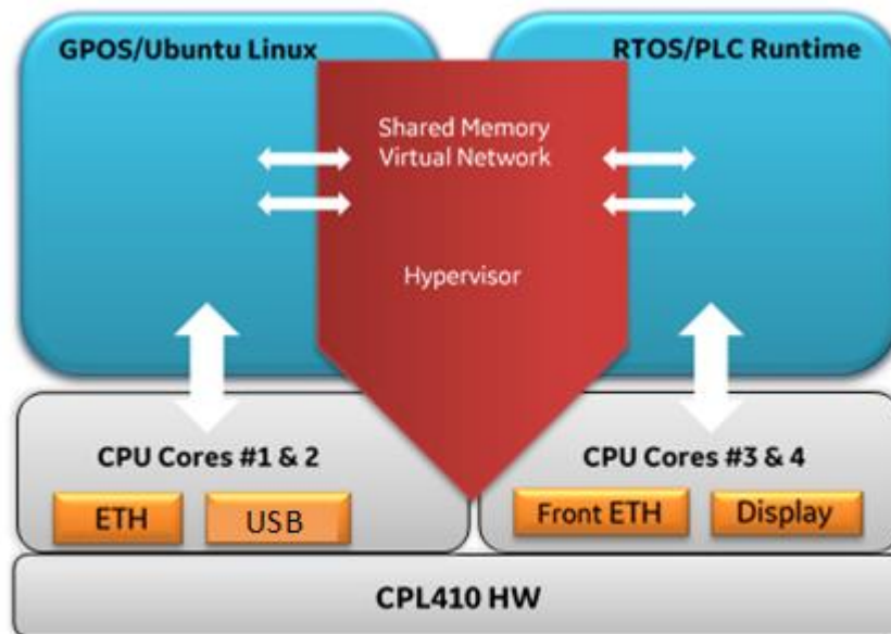
Figure 3: CPL410 Hardware/Software Separation
