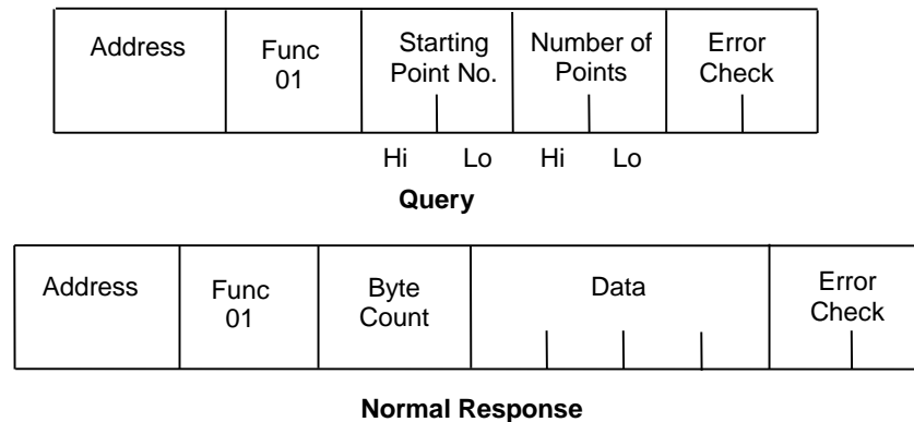
Figure 57: RTU Read Output Table Message Format
