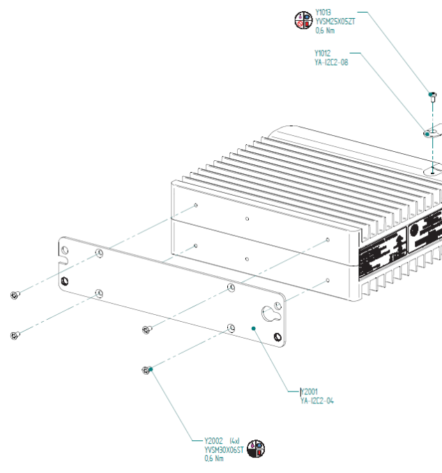
Figure 22: Panel-Mount Bracket Assembly CPE400
