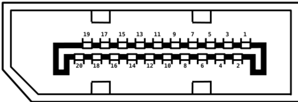
Figure 19: Display Port Connector
