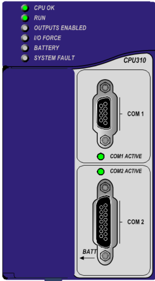
Figure 33: IC695CPU310 Front View
