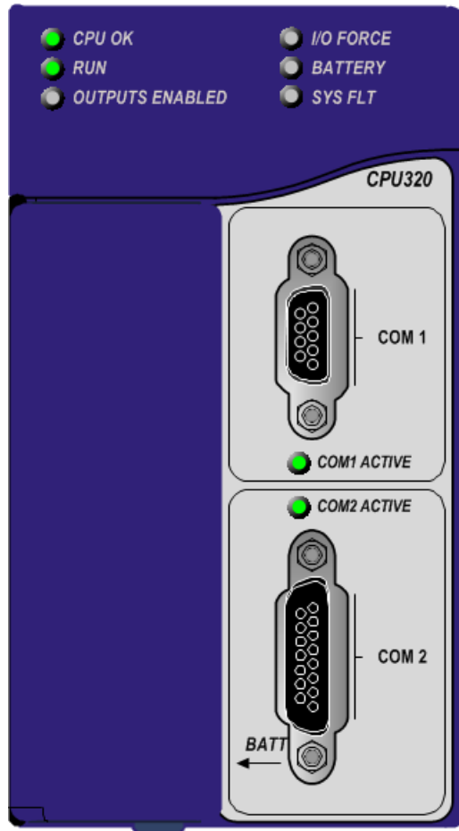
Figure 32: IC695CPU320 Front View
